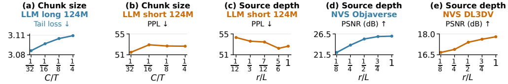
Figure 7: Chunk-size and source-depth ablations. (a,b) 124M long- and short-context LLM chunk-size sweeps; (c) 124M short-context LLM source-depth sweep; (d,e) NVS source depth on Objaverse and DL3DV. In (b,c), circles show WikiText PPL. C128 and source layers 0/3/9 use H200 runs; other short-context points use H100 runs. C512 is an archived control; C1024 and the last-layer reference reuse Table 2. In (a), circles show tail PTL over zero-based positions 30,720–32,766. Source depth is r/L , with one-based source layer r ; the source-layer indices above are zero-based.
