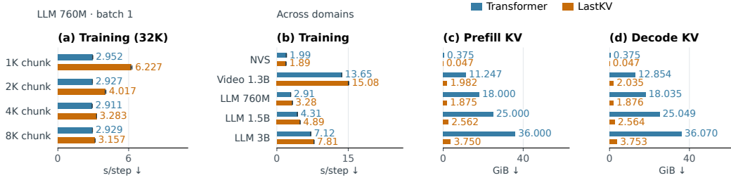
Figure 5: Measured efficiency. (a) 760M training at 32K, batch one; only LastKV varies chunk size. (b) Training across domains. (c,d) Physical self-attention KV after prefill and cached decoding. LLMs in (b–d) use 32K for training and 128K for inference, with C4K. Blue: Transformer; orange: LastKV. KV excludes weights/workspaces; whiskers span repetitions or block/scene medians.
