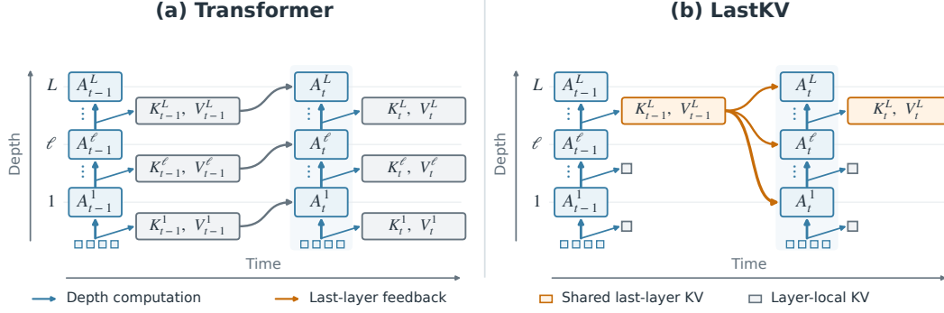
Figure 1: LastKV allows recurrence across time and depth. (a) Standard Transformer: At time step t , each layer \ell computes its attention readout A_t^\ell by retrieving the historical keys and values K_{t-1}^\ell, V_{t-1}^\ell (gray arrows) of previous tokens at the same layer. (b) LastKV: Every layer \ell at step t instead attends directly to the shared last-layer states K_{t-1}^L, V_{t-1}^L from step t-1 (orange arrows), routing deep completed representations of past tokens back into shallower layers of future tokens.
