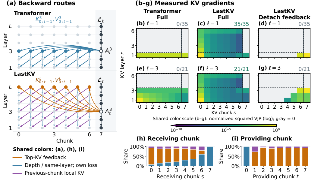
Figure 2: Recurrence and gradient flow in LastKV. (a) Backward paths from A_t^3 —the output of layer-3 attention for chunk t —to historical KV: a standard Transformer reaches only same- or lower-depth history, while LastKV also reaches last-layer states r = L through feedback. (b–d) VJP magnitudes from A_t^1 to historical KV for Transformer, LastKV, and LastKV with detached feedback (uses the same historical last-layer KV in the forward pass, but applies stop-gradient to it); (e–g) show the same comparison for A_t^3 . Only LastKV with differentiable feedback exhibits nonzero gradients to higher-layer historical KV. (h) Decomposition of the gradients received by each historical chunk s : blue denotes supervision from the chunk’s own loss through standard depth/same-layer paths, orange denotes feedback through the shared last-layer KV, and purple denotes the previous-chunk layer-local KV path. (i) The same decomposition from the perspective of the loss-providing chunk t , showing how supervision from later chunks propagates backward to earlier chunks. Together, these results show that the shared last-layer KV acts as a differentiable recurrent state, enabling BPTT-like credit assignment across both time and depth. Please refer to Appendix A for more details.
