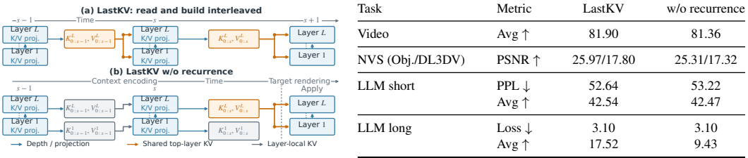
Figure 8: Recurrence ablation. (a) In LastKV, each completed chunk immediately shares its last-layer KV with all layers of subsequent chunks, so deep historical representations recurrently participate in constructing future context. (b) The nonrecurrent control instead constructs the context with standard layer-local attention and shares the resulting last-layer KV only when processing the final target. Thus, both variants provide the target with last-layer historical KV, while only LastKV recurrently reuses it during context construction. Right: recurrent feedback improves video/NVS quality and downstream LLM accuracy; long-context tail loss remains comparable. Video uses 1.3B models and LLMs use 124M models; PPL/Avg denotes WikiText perplexity/ten-task accuracy, and Loss/Avg denotes 30K+ tail loss/mean RULER.
