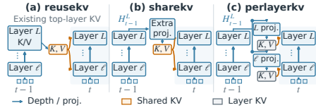
Figure 9: KV construction. (a) reusekv , (b) sharekv , and (c) perlayerkv , each at two times. Table 12 compares their NVS, LLM, and video results.
