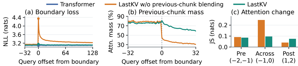
Figure 3: Previous-chunk blending mitigates chunk-boundary artifacts. (a) Next-token NLL aligned at chunk boundaries. LastKV without blending exhibits an obvious boundary spike, which is substantially reduced with blending. (b) Attention mass assigned to the immediately preceding chunk around the boundary; without blending, the abrupt switch from layer-specific to last-layer KV produces a sharper change in attention. (c) Jensen–Shannon divergence between the attention distributions of adjacent queries before, across, and after the boundary, showing that blending reduces the across-boundary discontinuity.
