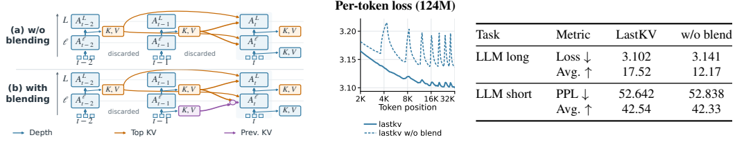
Figure 6: Previous-chunk blending. Left: historical KV available at t , (a) without and (b) with blending (circles). Chunks s \leq t - 2 retain only last-layer KV; earlier attention reads are omitted. Center: 124M per-token loss for LastKV (solid) and LastKV w/o blend (dashed) by token position (log-scaled axis, positions below 2K omitted, 768-token running mean); the periodic peaks without blending fall at the 4K chunk boundaries. Right: 124M long- and short-context comparisons using direct last-layer KV reuse.
