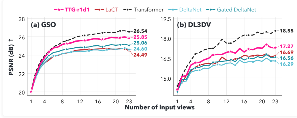
Figure 6: Per-view reconstruction quality on (a) GSO and (b) DL3DV. Curves show PSNR as input views accumulate for TTG ( r=d=1 ), LaCT, Transformer, DeltaNet, and Gated DeltaNet. Pink stars denote TTG; end-point labels report the 24th view predicted from 23 inputs, rather than the mean across all prediction positions.
