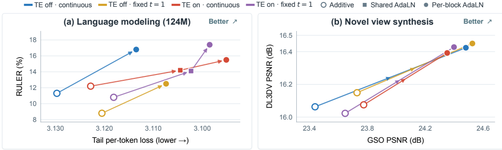
Figure 5: Conditioning ablations at r=d=1 . (a) Tail per-token loss and RULER accuracy; (b) GSO and DL3DV PSNR. Colors encode timestep embedding (TE) and time settings (plot t denotes noise level \rho ). Arrows connect additive conditioning (hollow circles) to per-block AdaLN (filled circles); the TE-on language-model paths include shared AdaLN (squares). Loss is reversed, so upper right is better.
