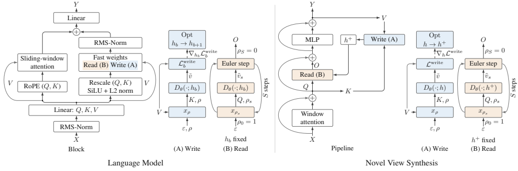
Figure 2: Language-model (left) and novel-view-synthesis (right) interfaces. Blue (A) accumulates weighted denoising losses into \mathcal{L}_b^{\text{write}} ; dashed arrows supply its gradient to Opt (Eq. 1). Orange (B) reads with frozen state: prefix h_b before the language-model chunk update, or updated scene state h^+ for target-camera queries. Scene-group indices are suppressed. Write repeats r are omitted; training uses d read steps and evaluation uses S .
