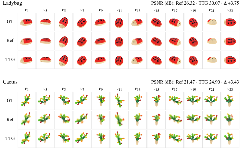
Figure 7: Full-set GSO reconstruction after writing all 24 views. Rows show ground truth (GT), deterministic reference (Ref), and TTG; columns select every other view index. Ladybug and cactus are selected high-gain examples highlighting markings and multi-part geometry, not benchmark averages. Gains of +3.75/+3.43 dB average all 24 targets, including observed views.
