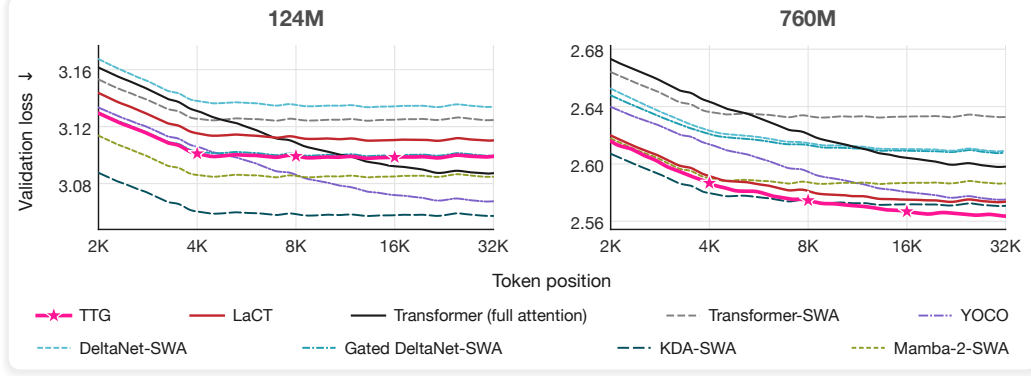
Figure A1: Per-token validation loss of TTG and eight baselines at 124M and 760M. The 760M DeltaNet-SWA and Gated DeltaNet-SWA curves are recovered, previously smoothed plot samples from the uTTT archive; the other 16 curves use complete numerical evaluation series. All inputs receive the same additional local smoothing for display on a logarithmic token-position axis from 2K to 32K. Recovered curves are not used to recompute scalar PTL. Stars highlight TTG; lower is better, with separate loss ranges for each size.
