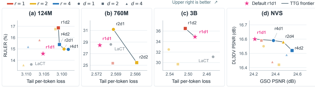
Figure 4: Pareto trade-offs across write repeats and trained readout depth. (a–c) Tail per-token loss versus mean RULER accuracy at 124M, 760M, and 3B. (d) GSO versus DL3DV PSNR. Colors encode write repeats r , and marker shapes encode trained readout depth d . Pink stars mark the default r1d1 configuration; gray points in (a–c) denote LaCT references. Lines connect nondominated configurations within each TTG sweep, while lighter points show the remaining results. Loss axes are reversed, so the upper right is better in every panel. Connecting segments serve as visual guides; the NVS frontier uses scores rounded to two decimal places.
