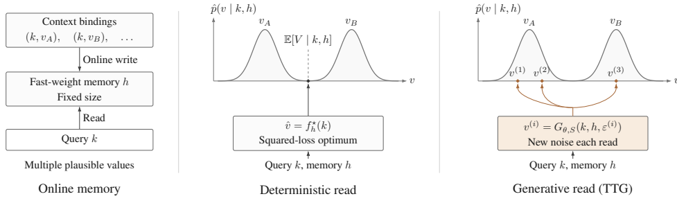
Figure 1: Readouts at matched fast-weight capacity. (left) Online writes form a fixed-size state h . (middle) The squared-loss optimum f_h^*(k) returns the conditional mean. (right) G_{\theta,S} samples with fresh noise and frozen h . Curves smoothly illustrate the discrete binding conditional. Mode recovery depicts a multi-step regime; at the Bayes optimum, S = 1 returns the mean.
